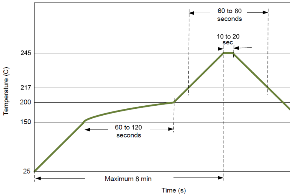
FIGURE 68: REFLOW SOLDERING
