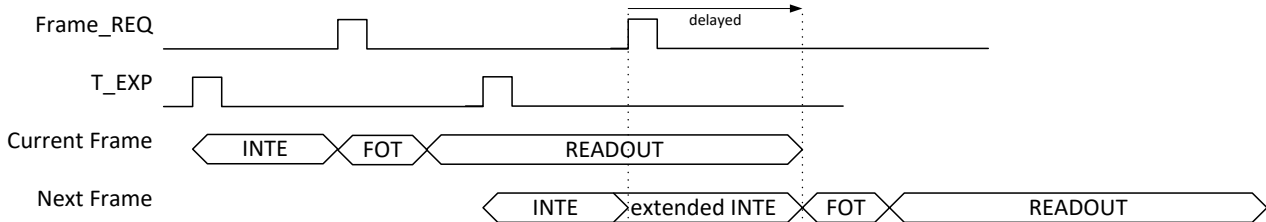
FIGURE 16: EXTENDED INTEGRATION TIME IN EXTERNAL MODE
