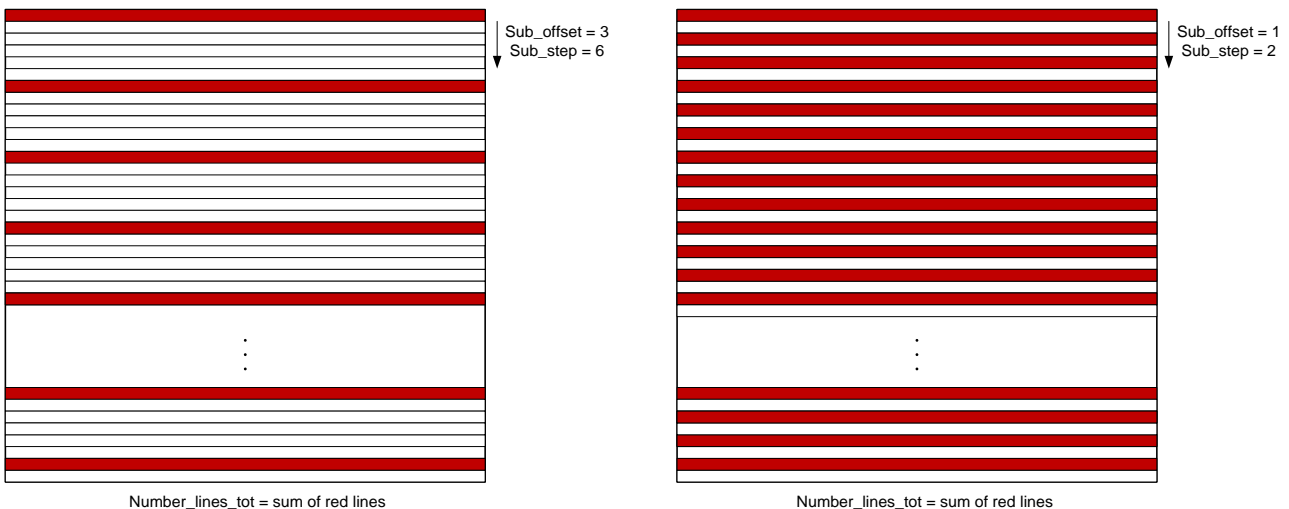
FIGURE 43: MONOCHROME SUBSAMPLING IN Y EXAMPLES (SKIP 5X AND SKIP 1X)
